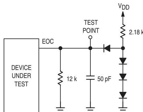
Figure 8. Test Circuit
